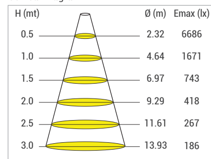
Conical Diagram
