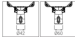
MK42: Ø42 MK60: Ø60
