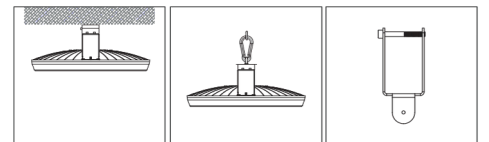
M01: Surface Cable Tray Mounting M02: Pendant Mounting M03: Busbar Hanger
